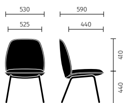
4 pieds, structure acier
