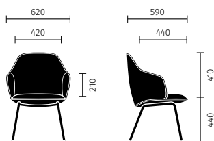
4 pieds, structure acier
