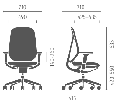
Dossier moyen Accoudoirs design 2D
