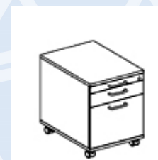
Mobile pedestal 9 U: height 592 mm, width 430 mm, depth 600/800 mm
