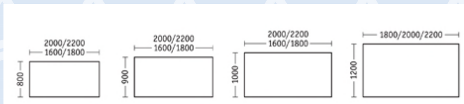
Desks / work tables (optionally with Returntable), table height 740 mm
