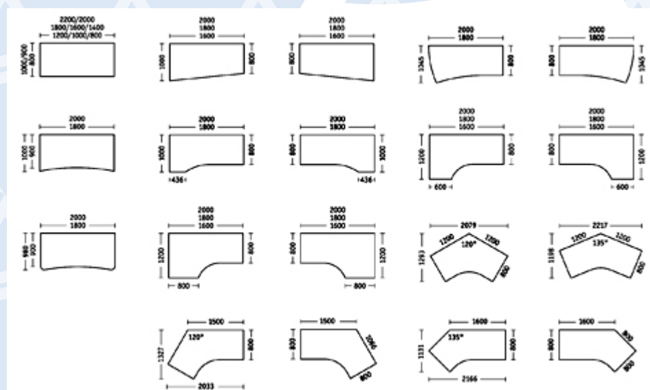
Desks / work tables
