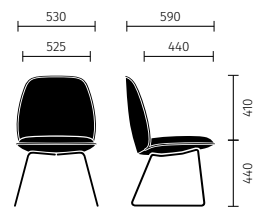
Skid base
